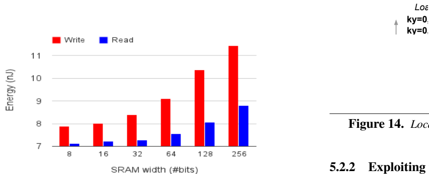
Figure 13. Read energy vs. SRAM width.
