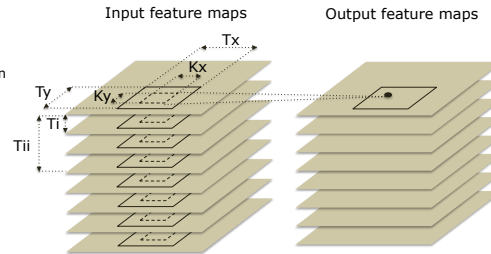
Figure 4. Pooling layer tiling.
