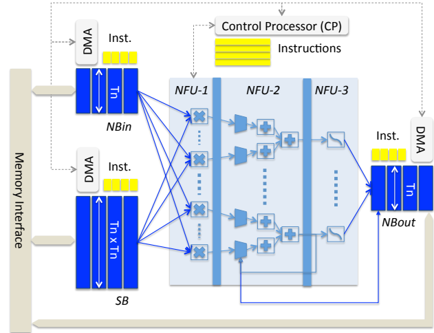
Figure 11. Accelerator.
