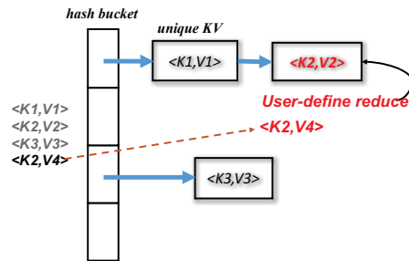
Fig. 6: Design of partial-reduction in Mimir.
